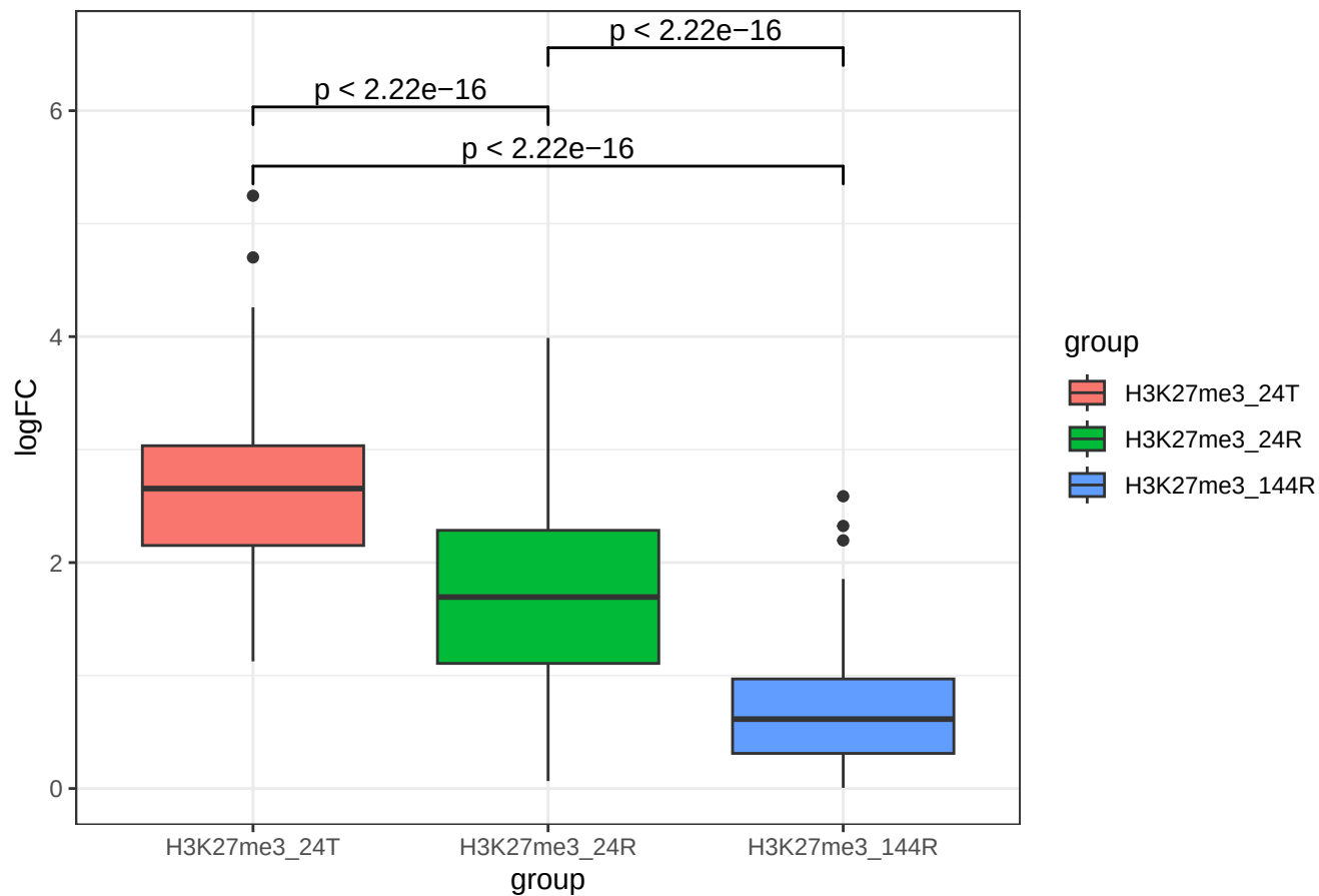
Absolute LFC across time for H3K27me3 set2
